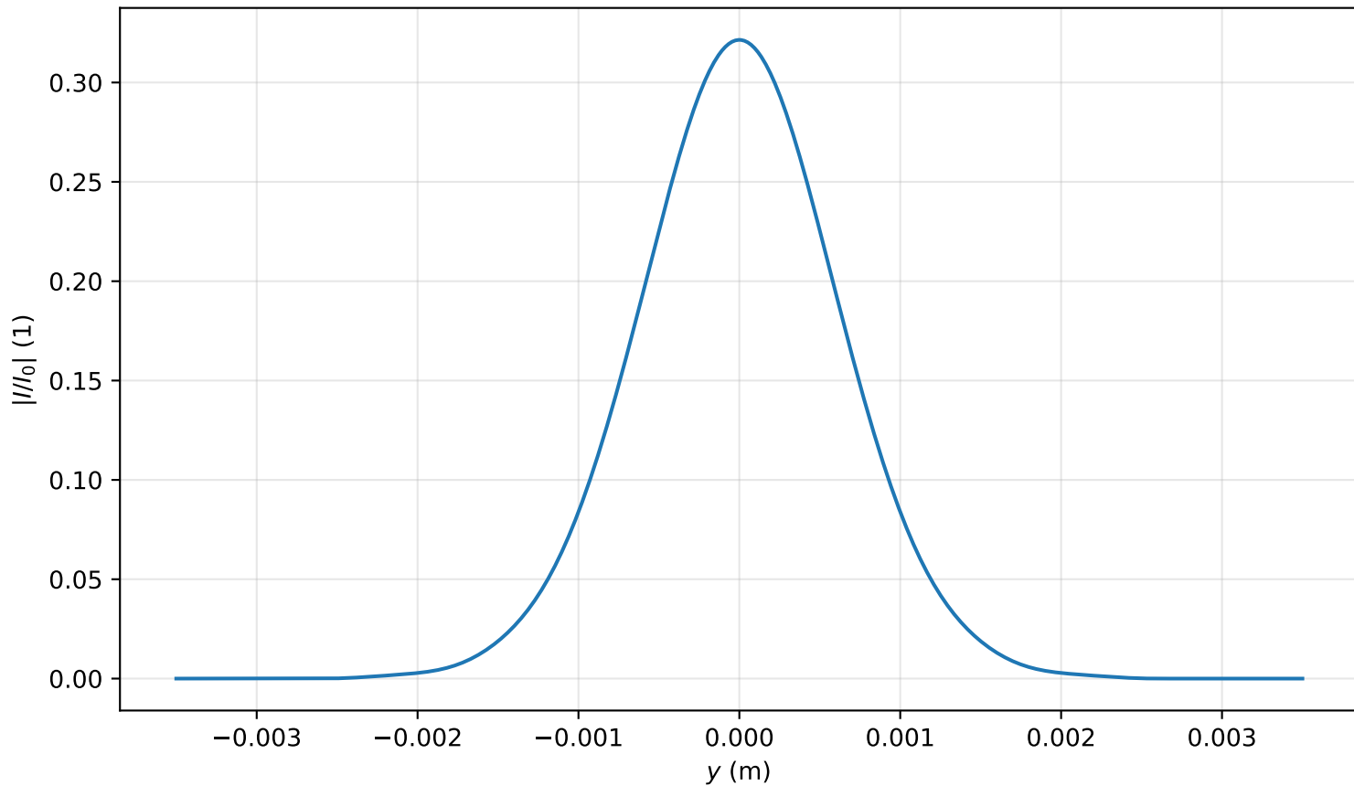
Intensity profile I(x=0, y, z=3.662)/I_0 , P_{in}=0.3P_{cr} , artificial time
